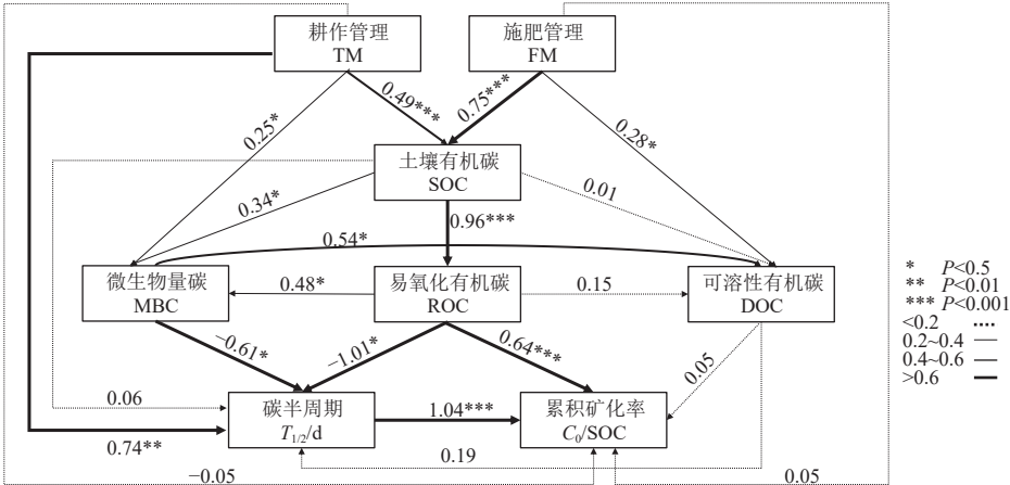
注：TM 为耕作管理；FM 为施肥管理；图中箭头上的数字为标准化路径系数。 Note: TM, tillage management; FM, fertilizer management; The numbers on the arrows are significant standardized path coefficients.
